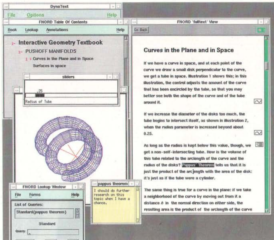
Figure 2: Running on a Unix workstation with Motif, the display includes a hierarchical table of contents window and a full-text view with several link icons. The reader has searched for the phrase "Pappus' Theorem" and clicked in the table of contents to scroll to the section on curves. The reader has followed a link to an external, interactive three-dimensional modeling program that illustrates the theorem. Finally, the reader has created an electronic note as a reminder to do additional research. The Brown University Graphics Group prepared this interactive textbook. (Courtesy of Electronic Book Technologies)
